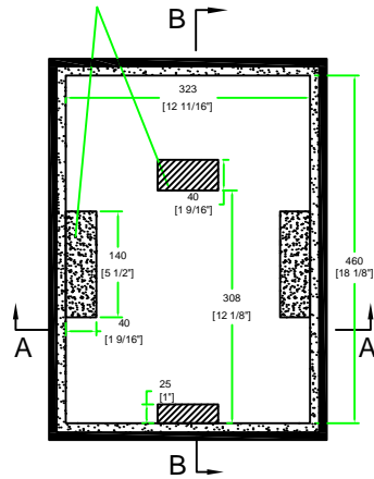
TOP VIEW OF COVER
