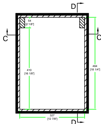
TOP VIEW OF BASE
